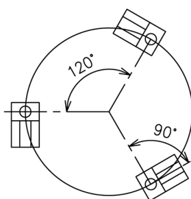
Tangential layout
